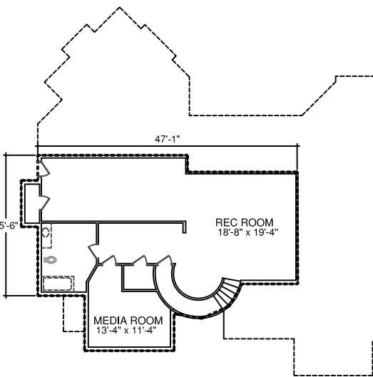
LOWER LEVEL
