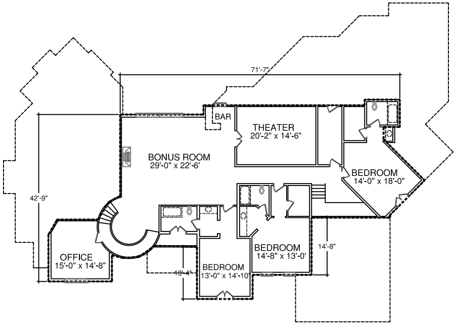
2nd FLOOR
