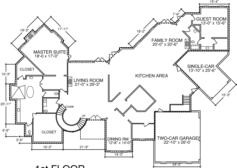
1st FLOOR
