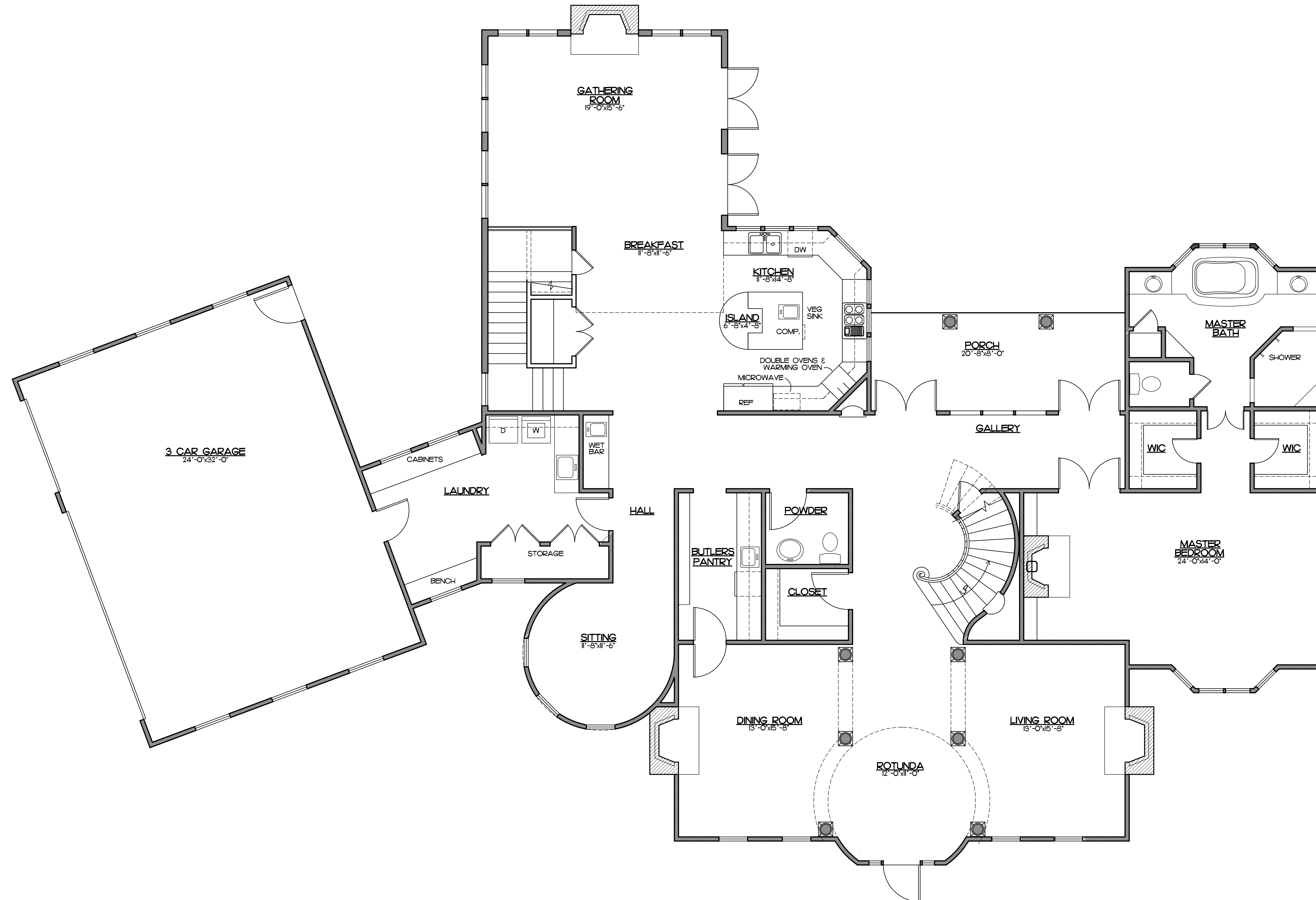
FIRST FLOOR PRESENTATION PLAN SCALE: 1/4" = 1'-0"
