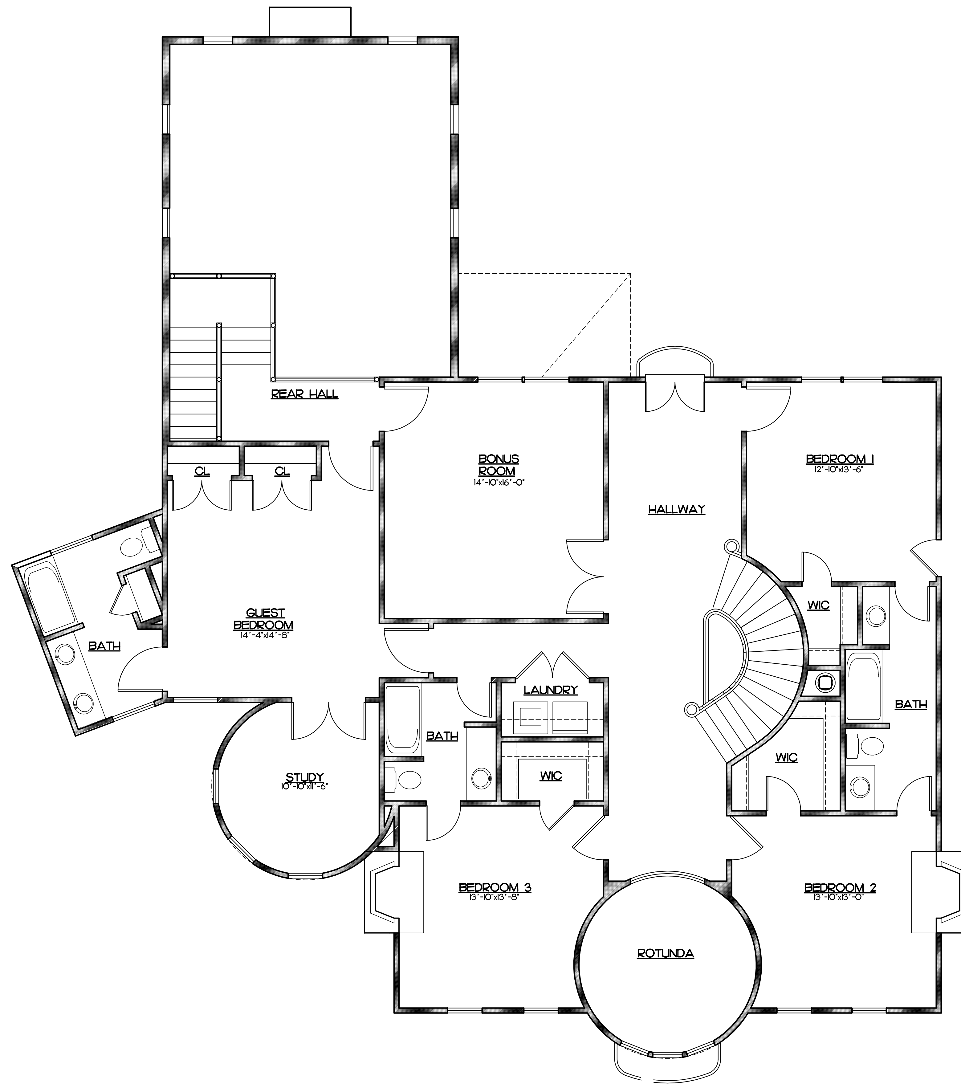
SECOND FLOOR PRESENTATION PLAN SCALE: 1/4" = 1'-0"
